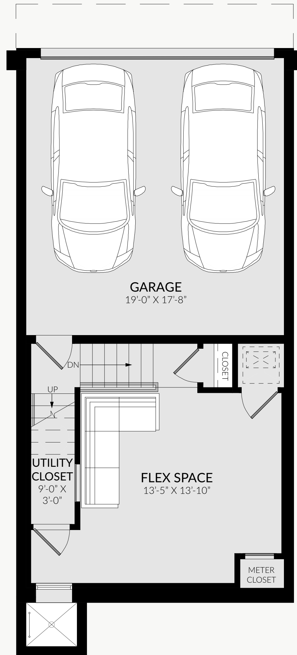
CELLAR/GROUND FLOOR PLAN
