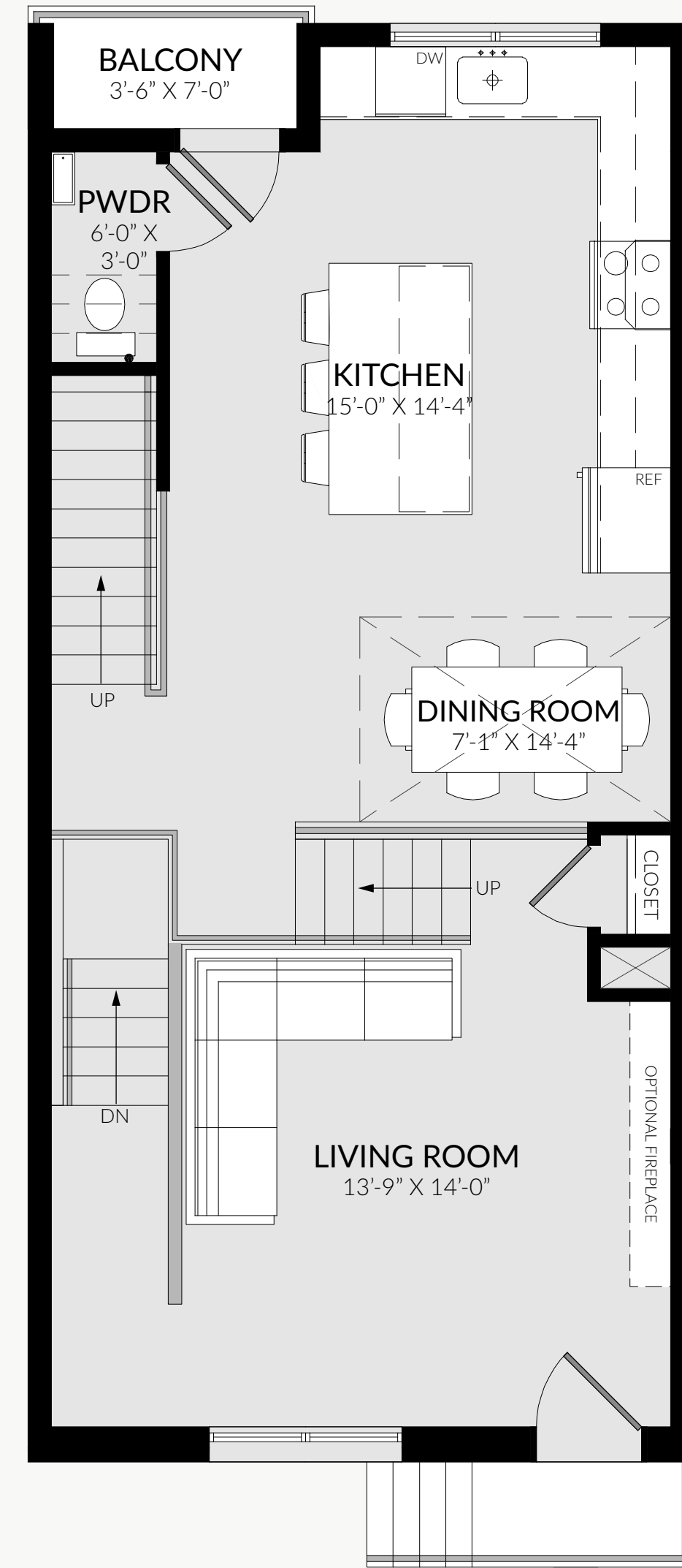
FIRST/SECOND FLOOR PLAN
